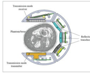
Schematic of rotating ultrasound transmitter
