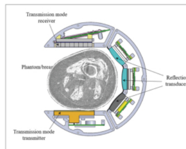
Schematic of rotating ultrasound transmitter
